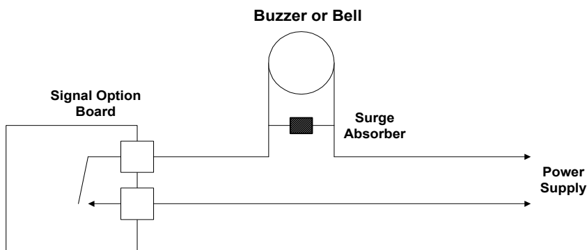
Figure – Time Signal Wiring Diagram
